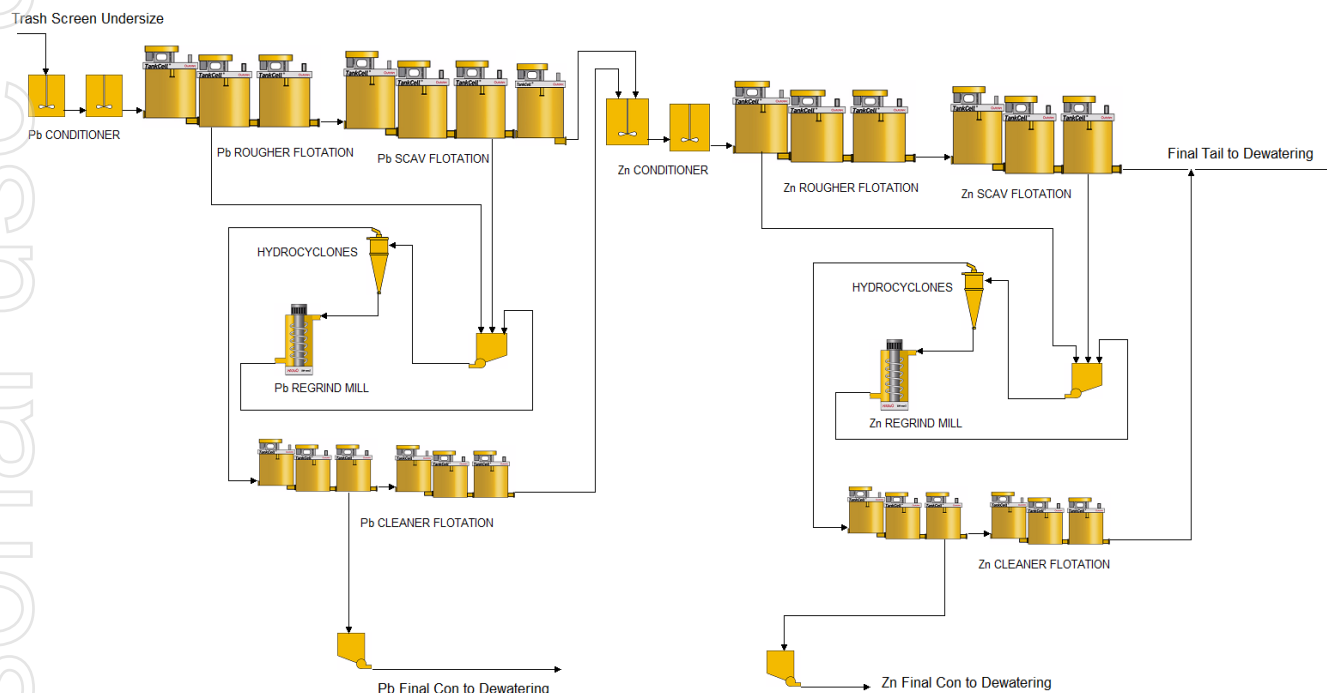
Figure 8. Flotation Flowsheet
