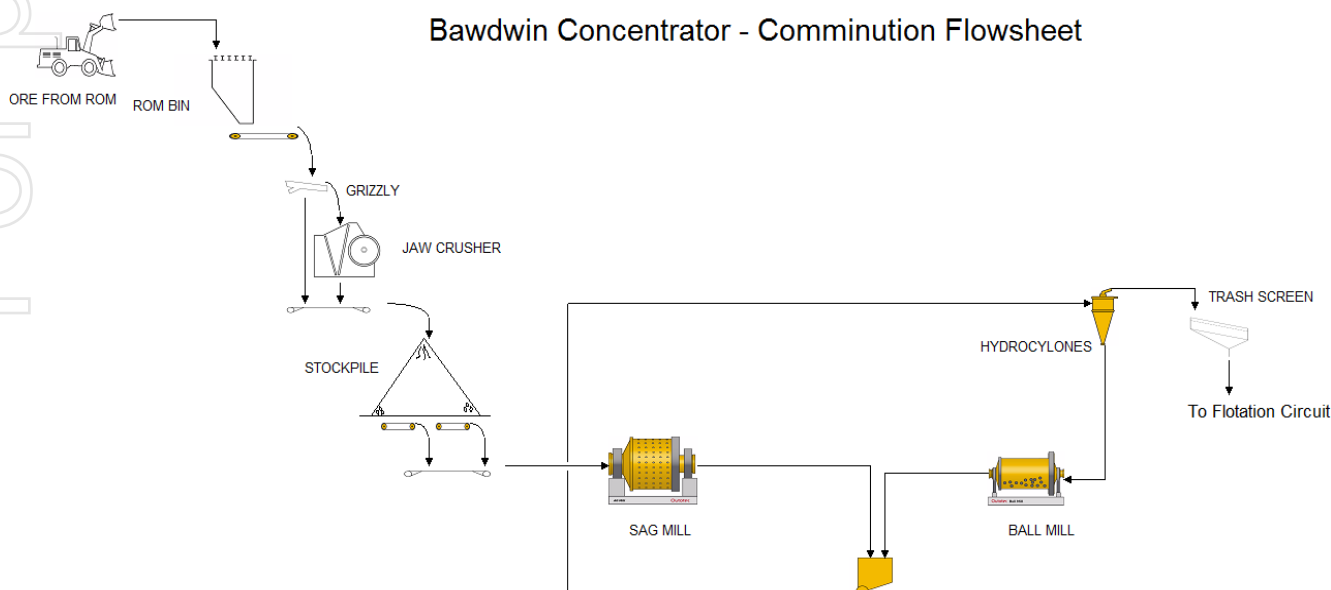
Figure 7. Comminution Flowsheet
